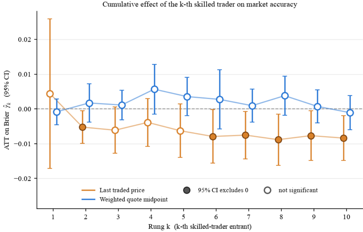
Figure 12: Difference in the time-weighted Brier score to close between markets ending with exactly k skilled traders and those ending with k - 1 .
