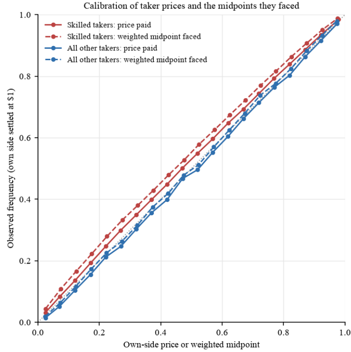
Figure 6: Observed frequency with which the taker’s side settled at $1, by own-side price paid (solid) and by the weighted midpoint faced (dashed), for skilled takers (red) and all other takers (blue). Bins of width 0.05, contract-weighted. The dotted line is perfect calibration.
