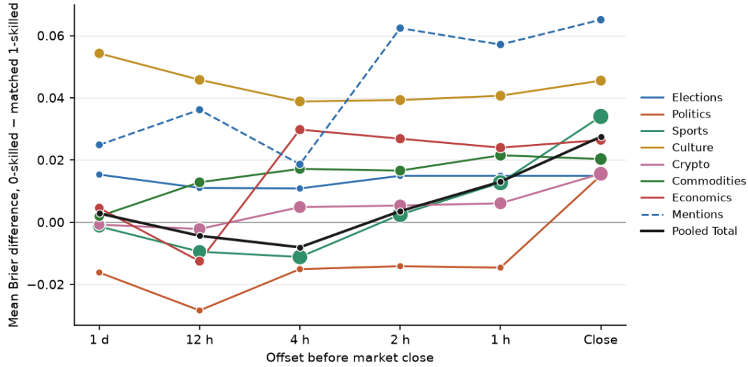
Figure 8: Mean difference in Brier score between markets with no skilled trader and matched markets with exactly one, by category and horizon before close. Markets are matched on exact series ticker, total volume within 20 percent, and lifespan within 10 percent. A positive value means the market with one skilled trader was more accurate. The black line pools all categories.
