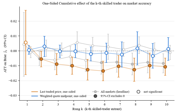
(b) One-sided markets
