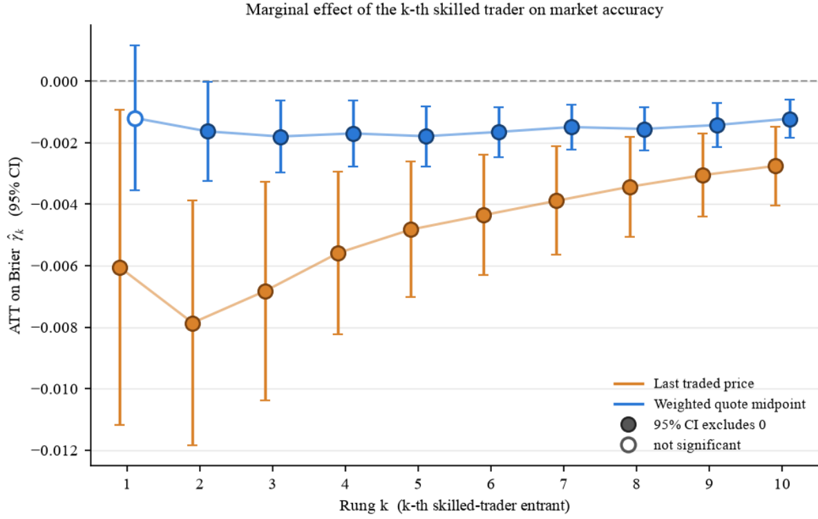
Figure 10: Change in the Brier score at the entry of the k -th skilled trader, relative to controls. Bars are 95 percent confidence intervals. Filled markers exclude zero.
